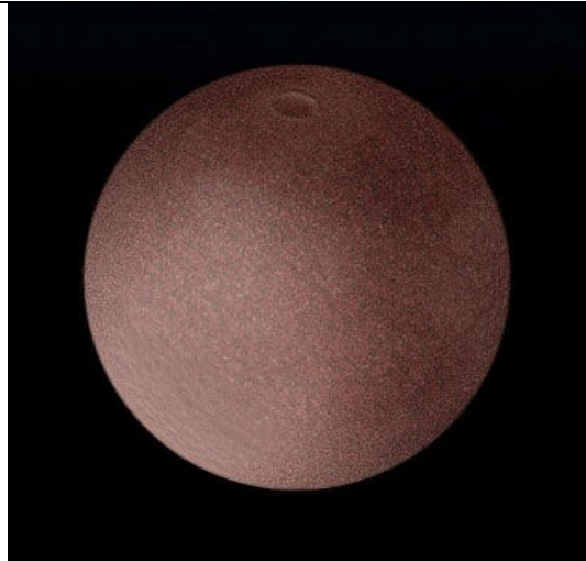
Makemake
