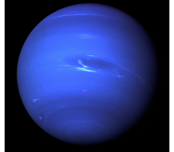
Neptune
